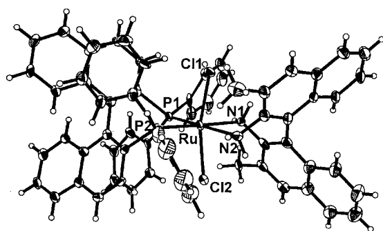
Figure 5. X-ray analysis of \text{RuCl}_2[(S)\text{-binap}][(S)\text{-dmdabn}] . Selective bond lengths [Å] and bond angles [°]: Ru – Cl1 2.418(4), Ru – Cl2 2.401(3), Ru – P1 2.273(3), Ru – P2 2.270(4), Ru – N1 2.228(9), Ru – N2 2.263(10); Cl1 – Ru – Cl2 165.34(11), P1 – Ru – P2 89.80(12), N1 – Ru – N2 80.1(4).
