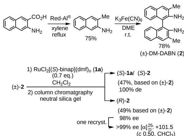
Figure 4. Synthesis of racemic DM-DABN 2 and enantiomer resolution with enantiopure BINAP-Ru(II) 1 .
