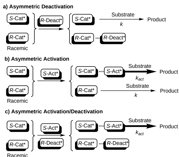
Figure 2. Strategies of asymmetric catalysis using a racemic catalyst.
