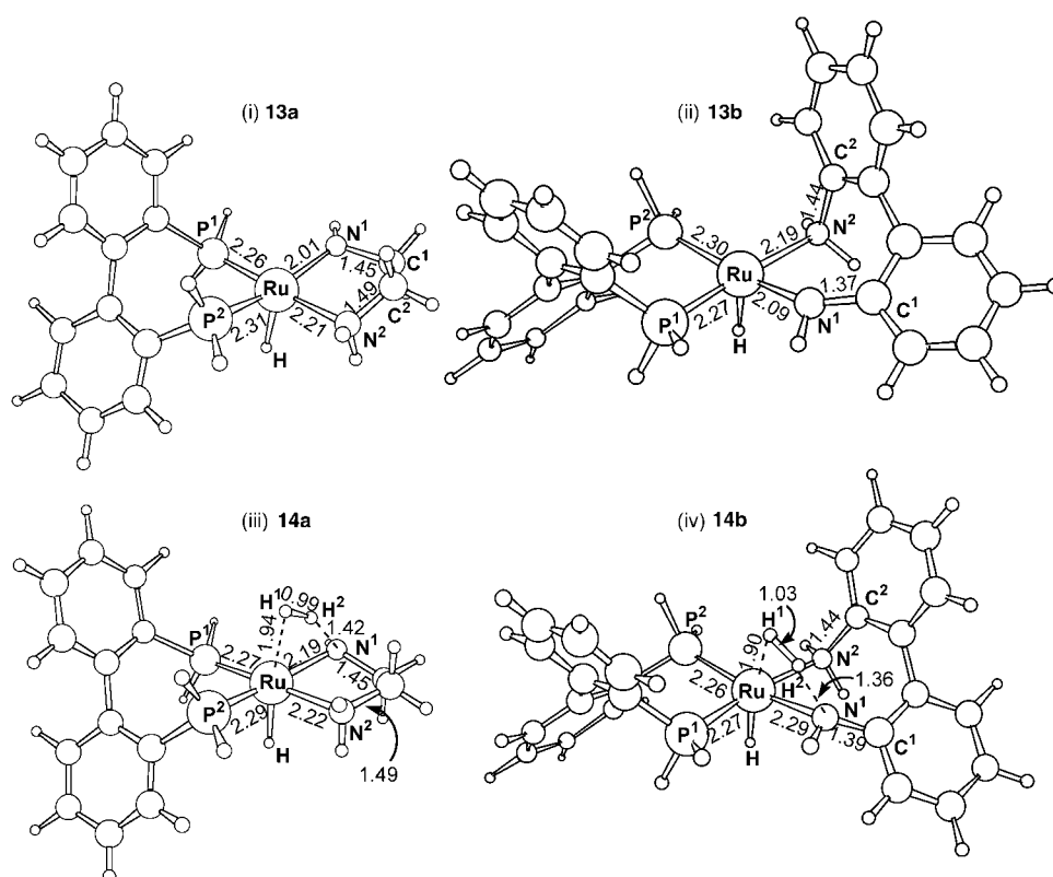
Figure 6. 3D structures of the amide complexes 13a and 13b (i and ii) and the hydrogen-splitting transition states 14a and 14b (iii and iv) at the B3LYP/631SDD level. Bond lengths are shown in Å.
