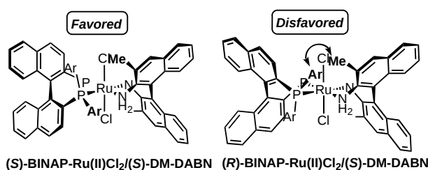
Figure 3. Rational design of a chiral deactivator for enantiomer discrimination of racemic BINAPs-Ru(II) complexes.
