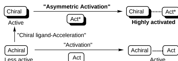
Figure 1. The concept of asymmetric activation.
