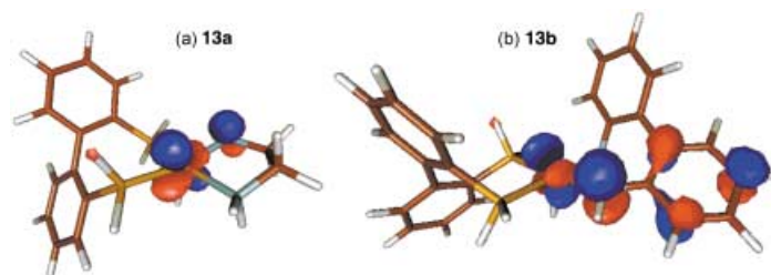
Figure 7. The highest occupied Kohn–Sham orbitals of 13a and 13b .
